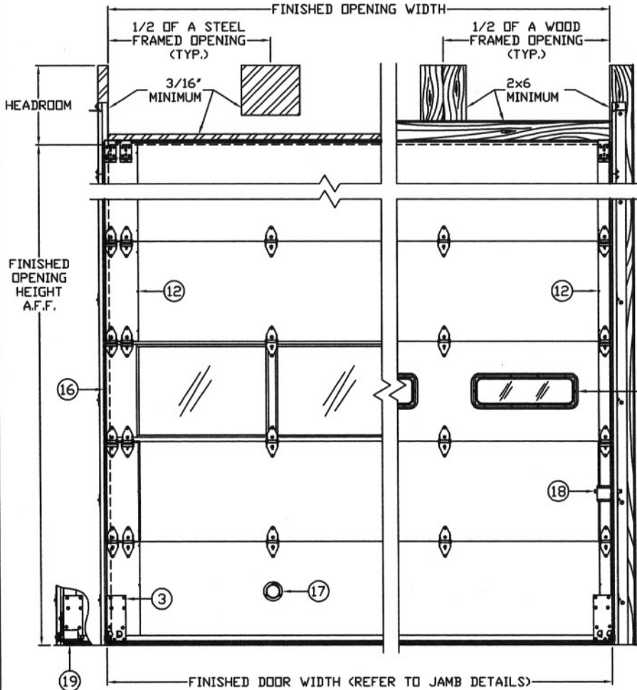
INTERIOR ELEVATION
